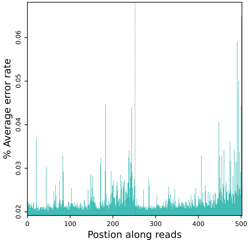
Error rate distribution along reads (R10508)
